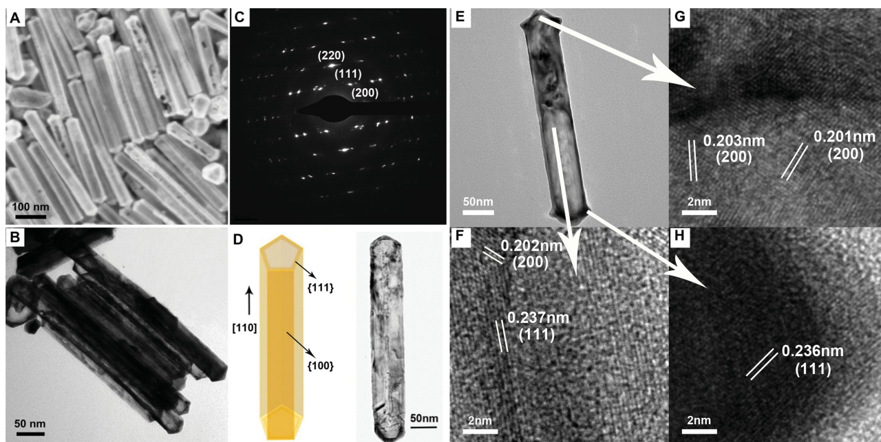
Figure 2. A) SEM and B) TEM image of Au NTs of length ≈370 nm; C) SAED pattern of an individual Au NT, D) schematic illustration of the elongated cyclic penta-tetrahedral model of Au NTs and real space (TEM) image; E) TEM image of a broken Au NT, of which the outer wall was partially detached, exposing the inner wall; F) HRTEM images of the inner wall, G) outer wall, and H) open end of the nanotube in (E).
